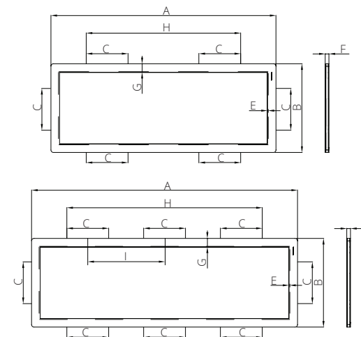
DIMENSIONS (mm)
