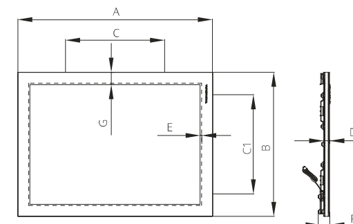
DIMENSIONS (mm)
